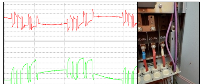
Figure 11: Cause of interference
