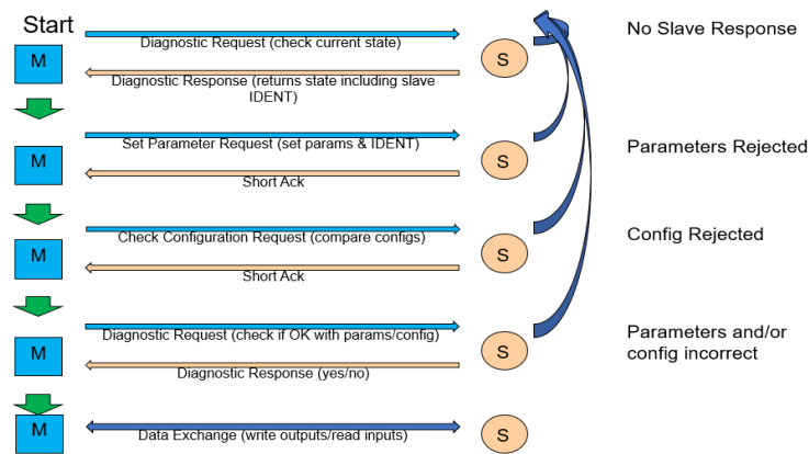
Figure 18: System start-up process
