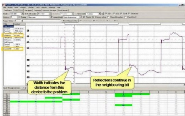
Figure 20: Oscilloscope reading when there is over termination
