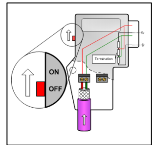
Figure 2: Termination on a connector
