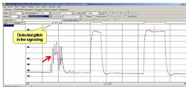
Figure 21: Oscilloscope reading when there is noise on the network
