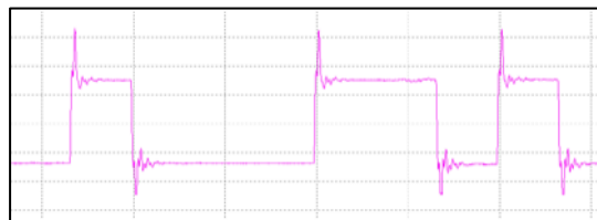
Figure 6: Missing termination waveform
