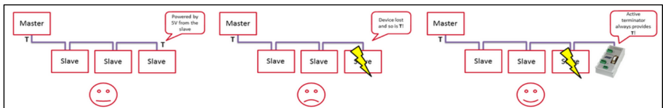
Figure 3: The difference between using an active terminator and terminating using modern
