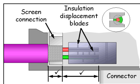
Figure 4: Guide for wiring into a Profibus DP connector
