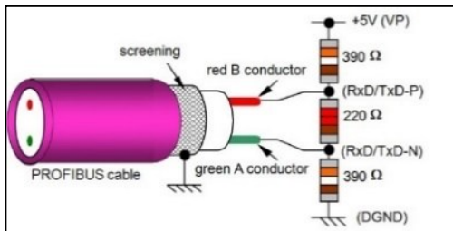
Figure 9: Active terminator
